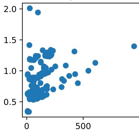
julia
