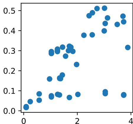
arith
