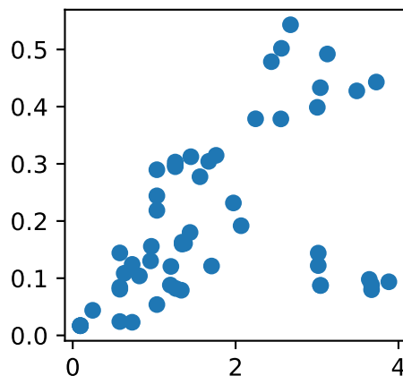
arith-fma
