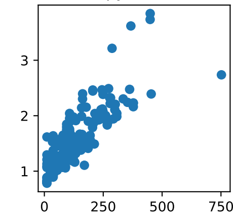
python
