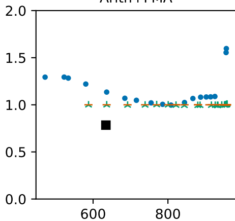
Julia
