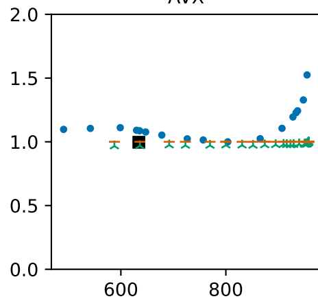
Python
